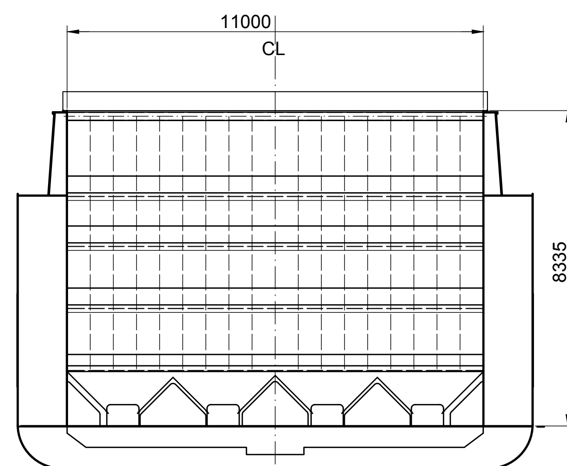
BULKHEADS #30 & #96
